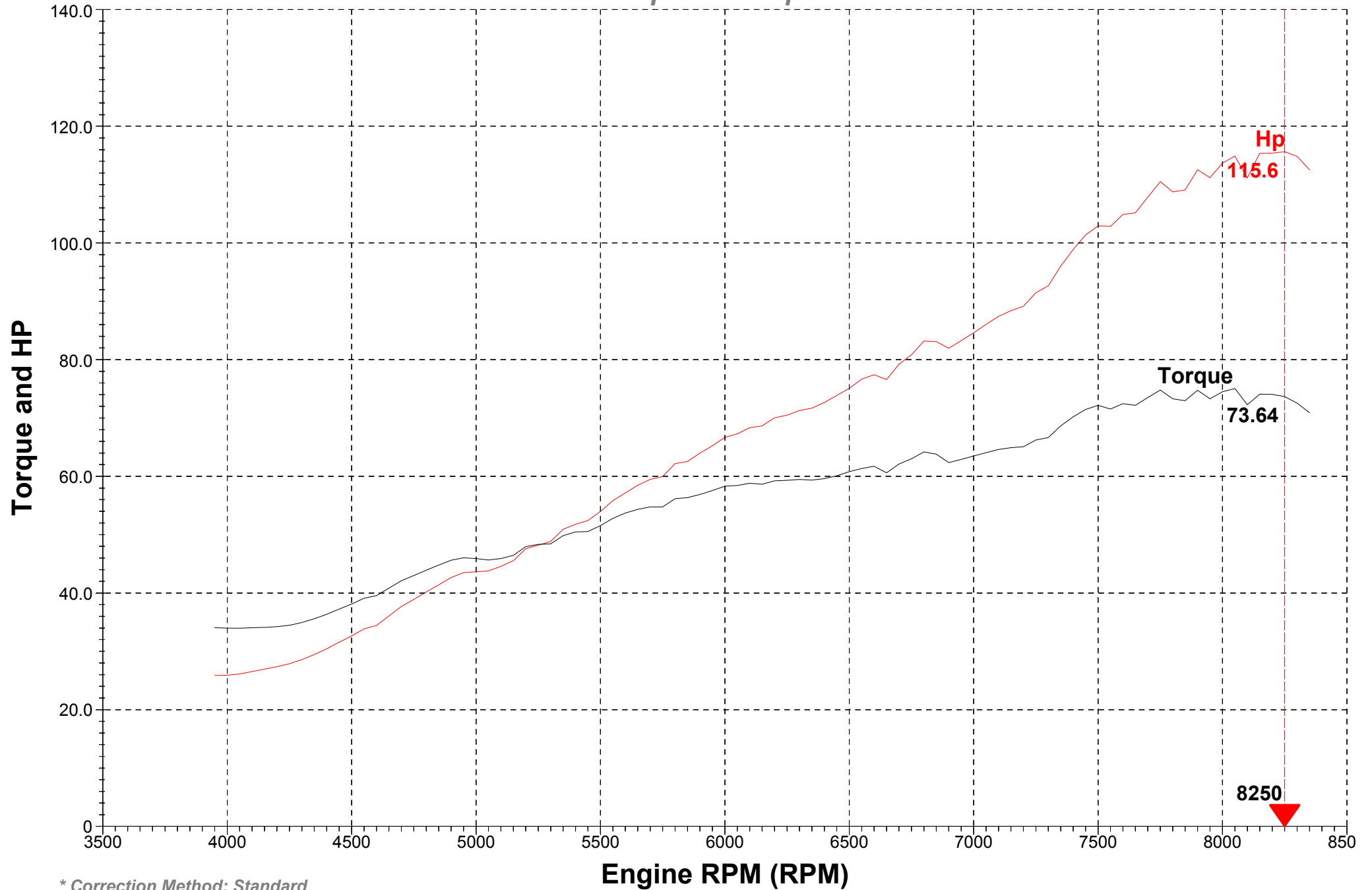
Peak Torque* and Hp* vs. RPM
