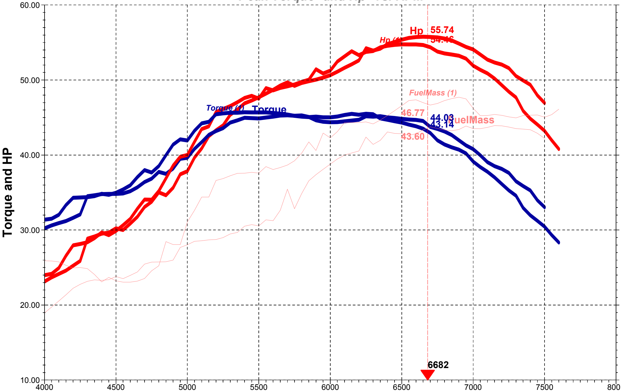
Peak Torque* and Hp* vs. RPM
